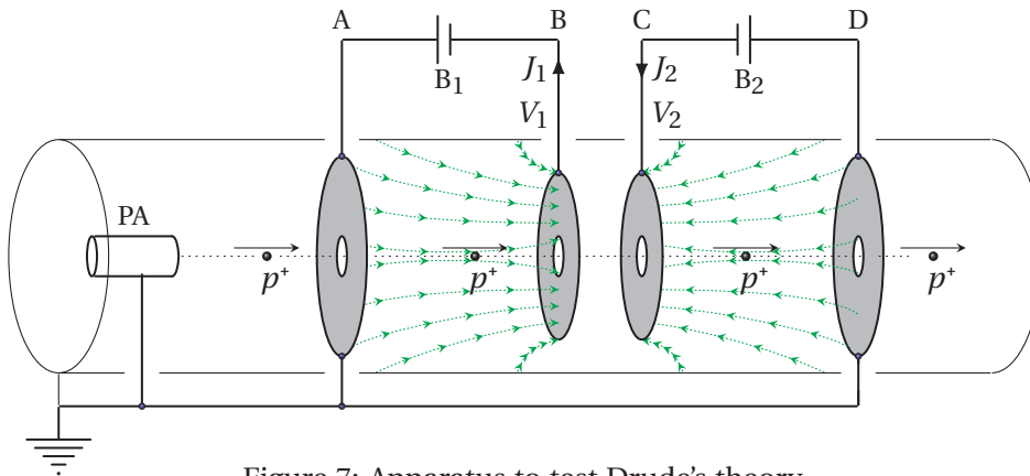
Figure 7: Apparatus to test Drude's theory.
