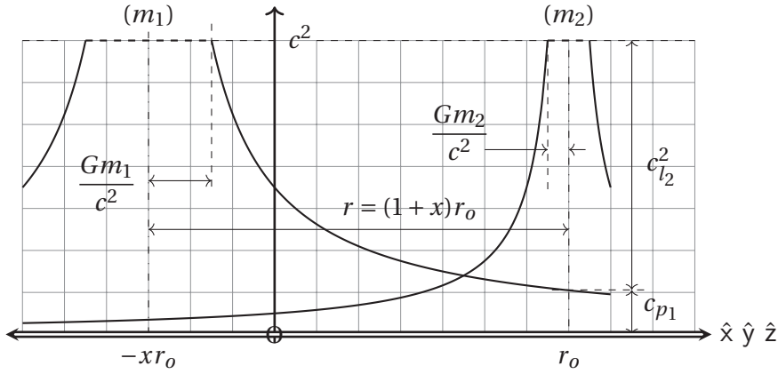
Figure 5: Transportivity, Gravitational Interaction, and Orbits . The horizontal axis represents the radially reduced space; the vertical axis represents transportivity, ranging from zero to c^2 . The figure illustrates the variation in transportivity resulting from the presence of two massive bodies, m_1 and m_2 , where m_2 = xm_1 , positioned symmetrically about their barycentre. The body m_2 perceives a local speed of light c_{l_2} = c^2 - c_{p_1} , where c_{p_1} is the transportivity deficit induced by the gravitational potential of m_1 . Although the diagram emphasises the effect of m_1 on m_2 , the interaction is fully reciprocal: each body induces a transportivity deficit influencing the other, and the forces satisfy F_{12} = F_{21} by construction.
