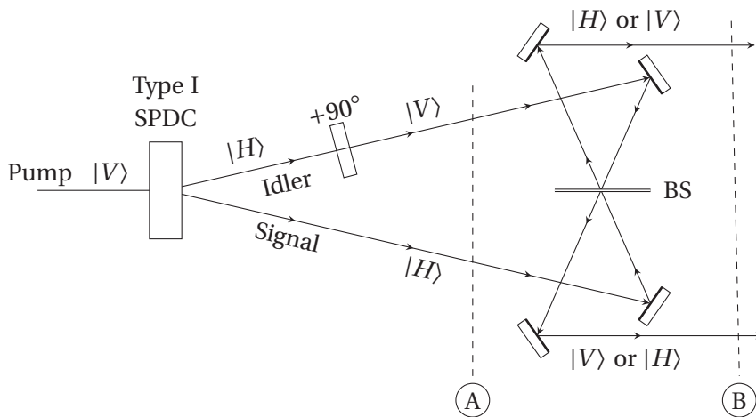
Figure 8: Ou and Mandel's experimental setup successfully demonstrating the violation of Bell's inequality at position B from a single type I SPDC.
