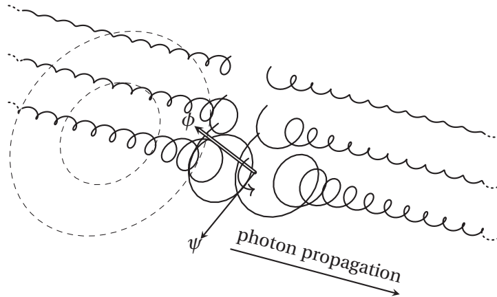
Figure 4: Schematic representation of the particle-wave duality of a photon in the R(3)SO(3) framework. The magnetic-like and electric-like field components gyrate within a quantised disc, projecting helical field structures with amplitudes decaying as 1/d and 1/r from the propagation axis. These nilpotent, non-energetic fields extend to infinity, signalling the photon's internal structural properties across space.
