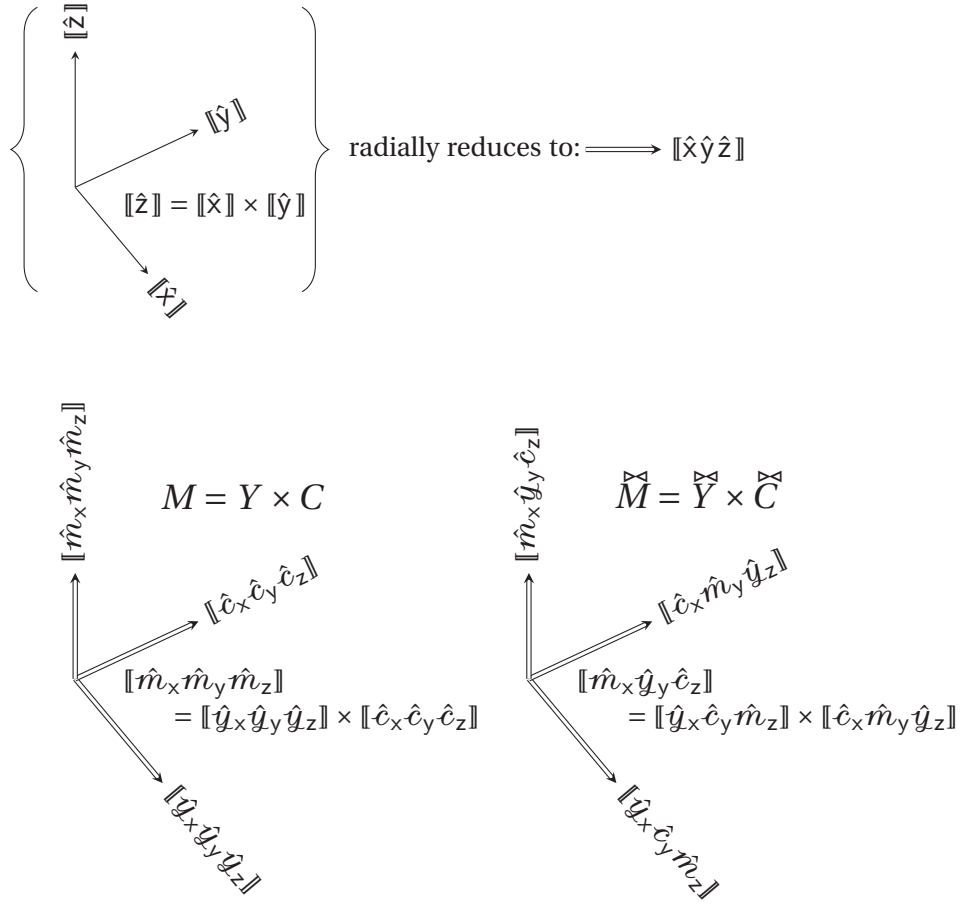
Figure 2: Visual representation of radial reduction applied to structured spaces. The top section illustrates the radial reduction of the space SO(3) \subset \mathbb{R}^3 to a single composite axis. The bottom-left section shows the eigenspaces M = Y \times C with their full set of radially reduced axes. The bottom-right section shows the potential space, in which the axes are consistently selected from each of the constituent spaces Y , C , and M according to the cross-product relations M = Y \times C , \tilde{M} = \tilde{Y} \times \tilde{C} , and \hat{z} = \hat{x} \times \hat{y} .
