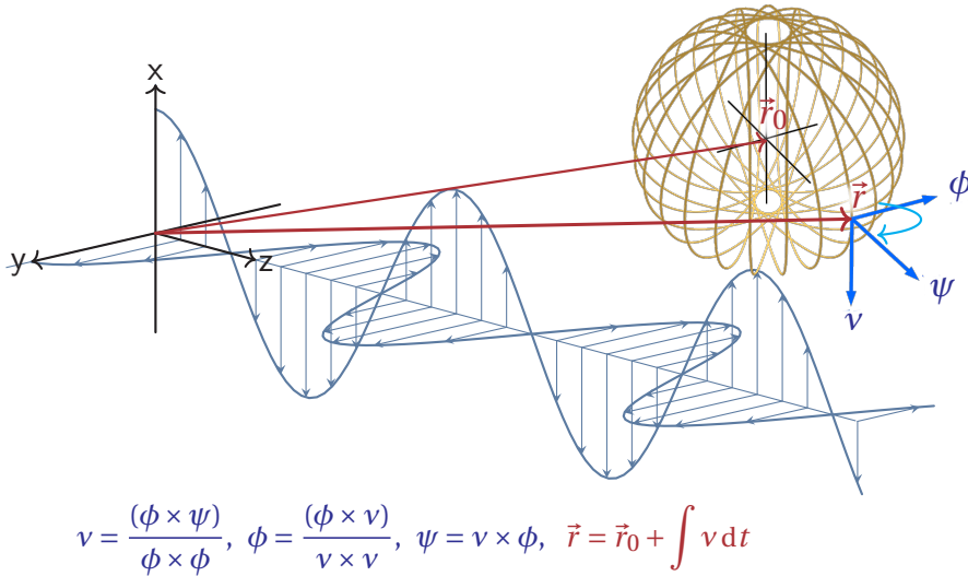
Figure 1: Here a travelling plane wave, with phase velocity c , is juxtaposed to a soliton described by the below solution of \mathcal{M} , both satisfying the Maxwell equations in vacuum. It is a gyration (spinning vortex) propagating with velocity \|\mathbf{v}\| = c along a spherular path defined by \vec{r} .
