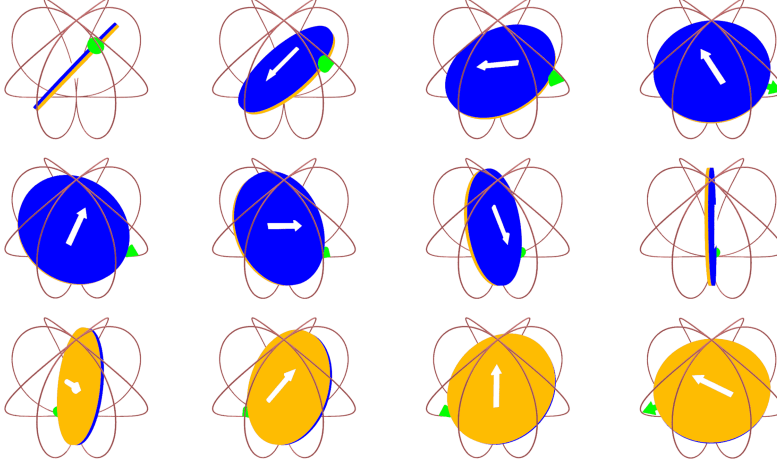
Figure 3: Visualisation of gyrations. The white arrow within the disc represents the magnetic vector (analogous to the second hand of a watch). The blue face indicates the forward-facing side of the disc, while the orange face indicates the rear-facing side; these coloured disc faces serve purely as visual aids to convey orientation and have no direct physical interpretation. The green pointer marks the 12 o'clock position and traces the indicated path. In the illustrated example, for each complete orbital period, there are four nutational periods. The sequence is generated with angular rates \omega_s = 5 , \omega_o = 1/2 , and \omega_w = 2 , requiring a full 4\pi rotation to complete one full cycle. This configuration models the composite spin, orbital, and nutational components inherent to the solitonic structure in R(3)SO(3) .
