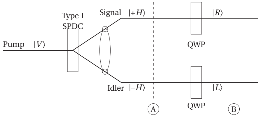
Figure 9: Schematic of the proposed experiment to distinguish field-based entanglement from collapse-based interpretations. A vertically polarised pump photon \Upsilon_0 undergoes Type I spontaneous parametric down-conversion, producing two linearly polarised photons: the signal in state |+H\rangle and the idler in |-H\rangle , differing by their solitonic rotation histories. Quarter-wave plates (QWPs), oriented relative to each soliton's internal polarisation frame, convert the signal and idler into right- and left-circular states |R\rangle and |L\rangle , respectively. To preserve entanglement symmetry and ensure valid nilpotent alignment \mathcal{U} + \bar{\mathcal{U}} = 0 , the optical path lengths to the QWPs should be equalised as closely as possible to maintain temporal coherence.
