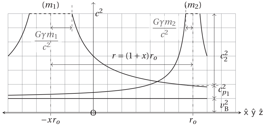
Figure 6: Boosted Orbits . This sketch builds on Figure 5 (pp. 81) to illustrate the effect of Lorentz boosting on a two-body system. Three key features are shown: (i) the boost-induced transportivity deficit v_B^2 appears as a constant offset; (ii) the energy levels of m_1 and m_2 undergo dilation due to boosting; and (iii) the transportivity curves flatten, becoming asymptotic to v_B^2 rather than to zero. The approach developed here for boosted orbits is structurally congruent with the treatment of ambient transportivity deficits. In environments with both ambient and boost-induced effects, the total deficit becomes v_B^2 \mapsto v_B^2 + v_a^2 .
